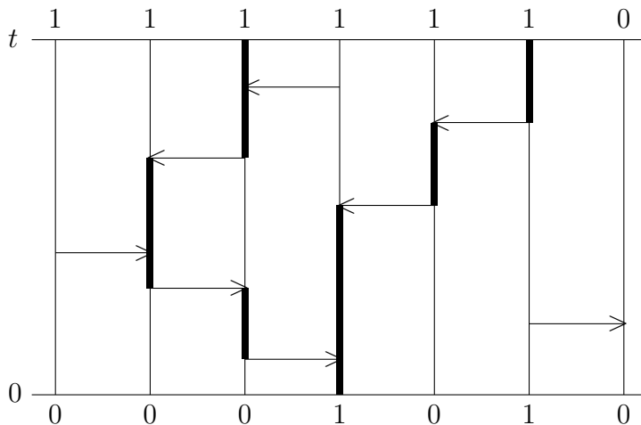
Figure 1: Voter model graphical representation and duality
