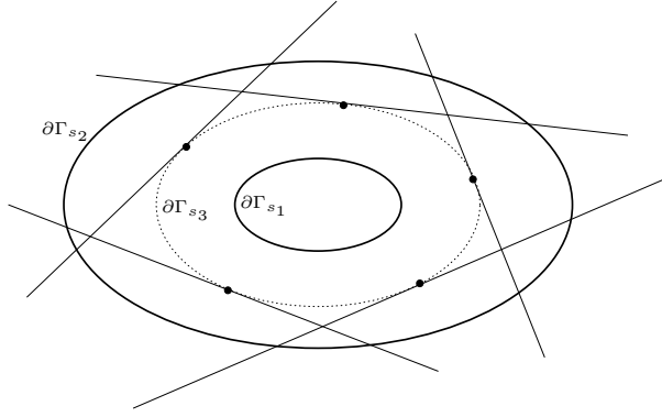
Figure 1: The convex sets \partial\Gamma_{s_1} , \partial\Gamma_{s_2} , and \partial\Gamma_{s_3} . The points represent c_j , j = 1, \dots, N_c , and the lines represent the sets \{c \mid \lambda_j \cdot (c - c_j) = 0\} . The region bounded by these line segments represents \bigcap_j \{c \mid \lambda_j \cdot (c - c_j) > 0\} .
