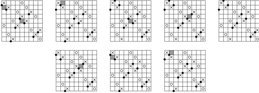
FIGURE 9. Finding states for the chain complex for P(-4, -3, 3) . The columns represent states in \mathfrak{B}_0, \mathfrak{A}_1, \mathfrak{B}_1, \mathfrak{A}_2, \mathfrak{B}_2 respectively. Shaded rectangles connect states in a given column to states in the next column.
