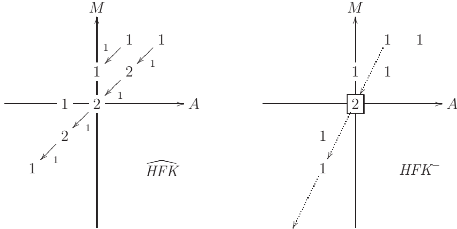
FIGURE 7. \widehat{HFK}(10_{132}) and HFK^-(10_{132}) . Large numbers represent ranks over \mathbb{F} . The arrows in \widehat{HFK} represent \delta_1 maps, with ranks shown; the dotted arrows in HFK^- represent multiplication by U . The invariant \theta lies in the boxed group.
