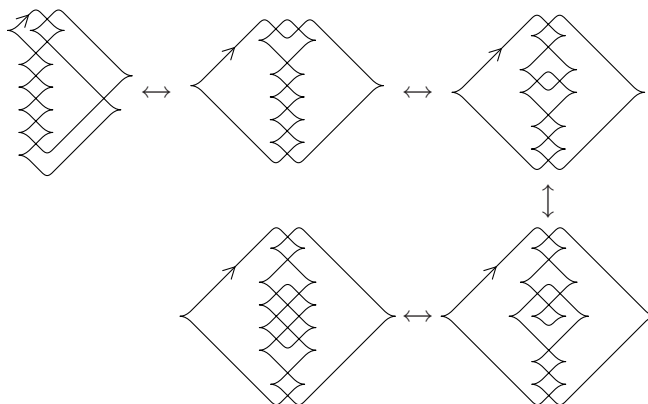
FIGURE 12. A Legendrian isotopy between G_2 and G_3 , the two forms of E(5, 1) . Starting from the upper left and moving clockwise, rotate (in the toroidal grid diagram) to the right one step, then rotate to the right and down two steps each, then perform a stabilization of type O:NW , and finally perform two commutations.
