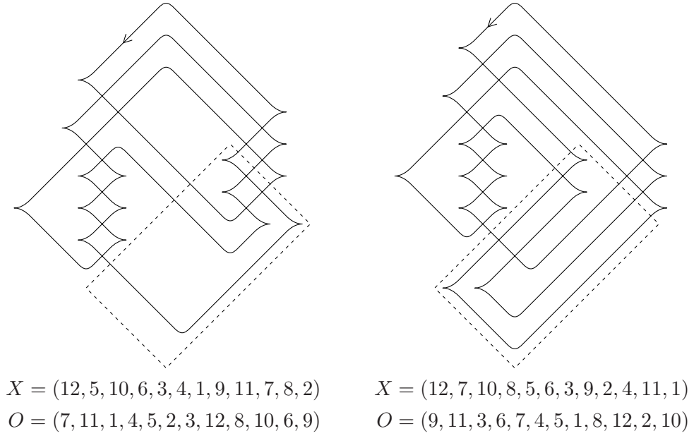
FIGURE 3. Legendrian m(12n_{200}) knots L'_1 (left) and L'_2 (right).
