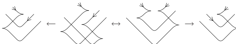
FIGURE 13. A local sequence of grid moves that goes from G_1 to G_2 . In the Legendrian category, these comprise a positive stabilization and destabilization. This same sequence can also be used to relate the Legendrian pretzel knot pairs and the Etnyre-Honda pair considered in Section 3.
