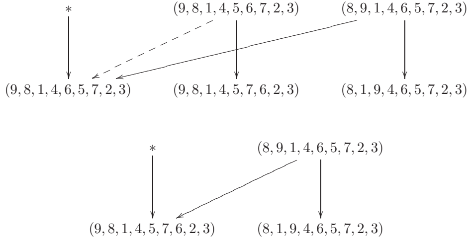
FIGURE 10. Contracting edges in the chain complex for P(-4, -3, 3) . At the first stage of building the complex for P(-4, -3, 3) , we obtain the complex pictured on the top. Here, the asterisk denotes the distinguished element a_0 . Contracting the dotted edge, we obtain the second complex, shown on the bottom.
