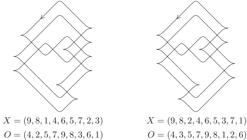
FIGURE 4. Legendrian P(-4, -3, 3) pretzel knots L_1 (left) and L_2 (right).
