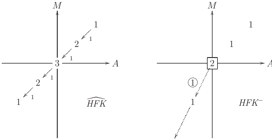
FIGURE 8. \widehat{HFK}(P(-4, -3, 3)) and HFK^-(P(-4, -3, 3)) . The invariant \theta lies in the boxed group, \delta_1 \circ \theta in the circled group.
