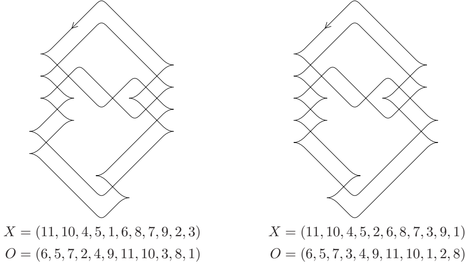
FIGURE 5. Legendrian P(-6, -3, 3) pretzel knots L'_1 (left) and L'_2 (right).
