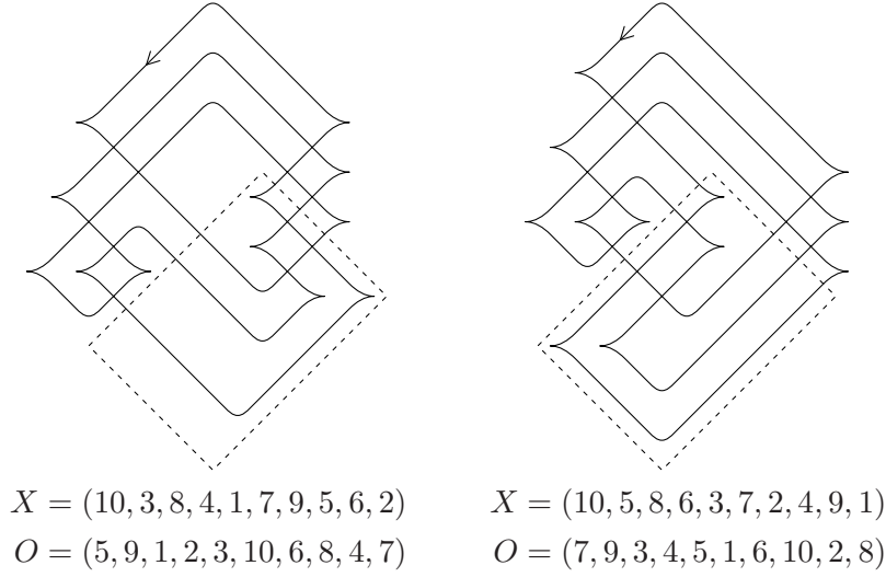
FIGURE 2. Legendrian m(10_{132}) knots L_1 (left) and L_2 (right). As pictured, these knots differ only in the dashed boxes, which are each topologically a negative half-twist on three strands.
