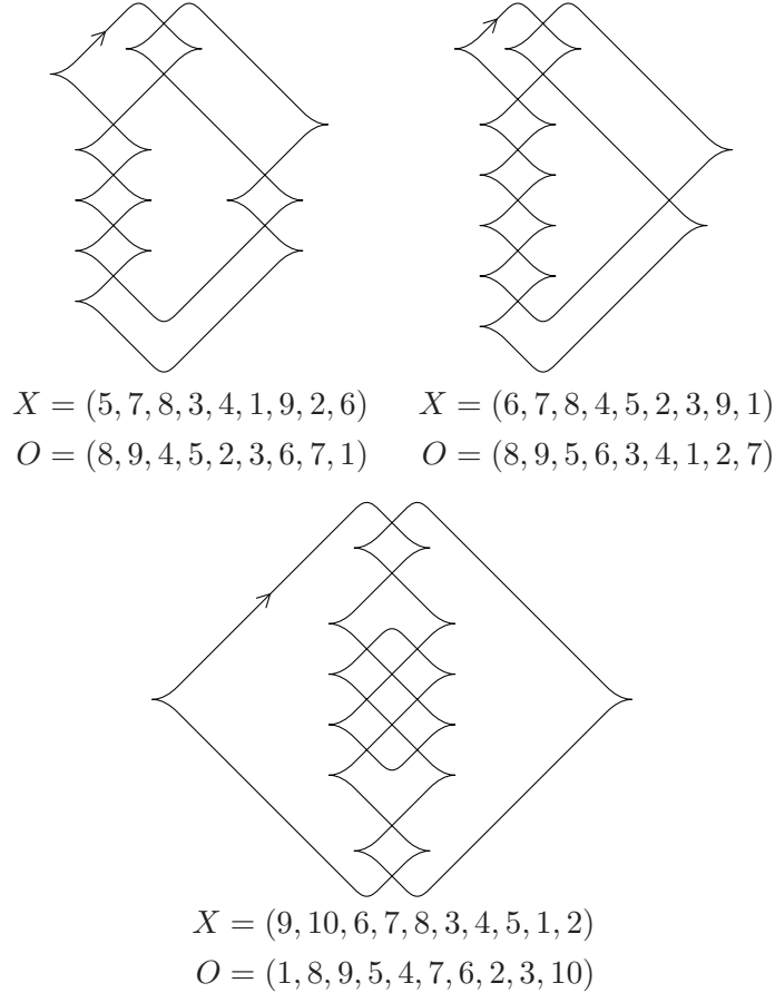
FIGURE 11. Legendrian knots from grid diagrams G_1 for E(2, 4) (top left) and G_2 for E(1, 5) (top right) of type 7_2 . An alternate, symmetric form G_3 of E(1, 5) is shown below.
