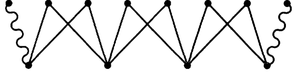
FIG. 1. Low pass filtering scheme for the ‘‘folded’’ case, going from V_{-3}^{\text{fold}} to V_{-2}^{\text{fold}} , in the case where support \phi = [-1, 2] , i.e., only h_{-1}, h_0, h_1, h_2 are \neq 0 ; in fact h_0 = h_1 = \alpha , h_{-1} = h_2 = \beta because of the symmetry conditions imposed (see text). The straight lines represent unaffected filter coefficients. In this case only two filter coefficients are affected by the folding (wavy lines—one at each end); the folded coefficient here is h_0 + h_{-1} = h_0 + h_2 .
