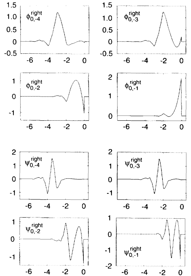
FIG. 7b. Same as in Fig. 7a for a right edge (i.e., on (-\infty, 0] ).
