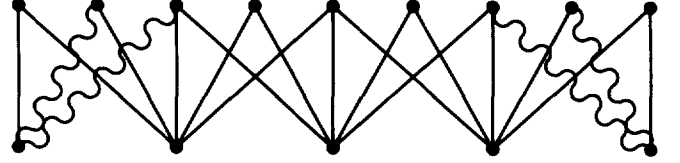
FIG. 2. Low pass filtering scheme for the “folded” case, going from V_{-3}^{\text{fold}} to V_{-2}^{\text{fold}} , in the case where support \phi = [-2, 2] , i.e., only h_{-2}, h_{-1}, h_0, h_1, h_2 are \neq 0 ; we have h_{-2} = h_2, h_{-1} = h_1 because of symmetry. This diagram corresponds to the unnormalized formula (2.12); some of the affected filter coefficients (wavy lines at edges) are equal to \sqrt{2} times their normal value in this case.
