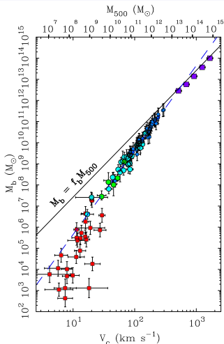
Figure: Total baryonic (regular) mass versus circular velocity. Each point represents a galaxy, including star dominated spirals (dark blue), gas dominated disks (light blue and green), Local Group dwarf satellites (red squares), except that the purple squares represent the mean of many galaxy clusters.
