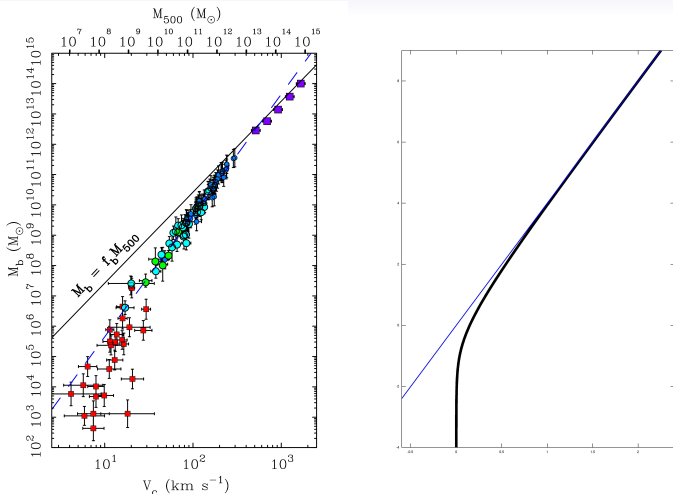
Figure: Total baryonic (regular) mass versus circular velocity. Each point represents a galaxy, including star dominated spirals (dark blue), gas dominated disks (light blue and green), Local Group dwarf satellites (red squares), except that the purple squares represent the mean of many galaxy clusters.
